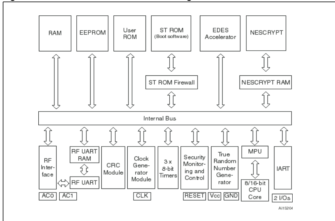
Figure 1. ST23YR48A / ST23YR80A block diagram
