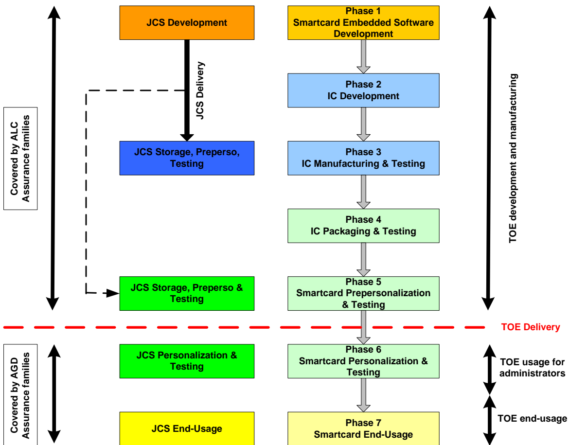
Figure 6: JCS (TOE) Life Cycle within Product Life Cycle
