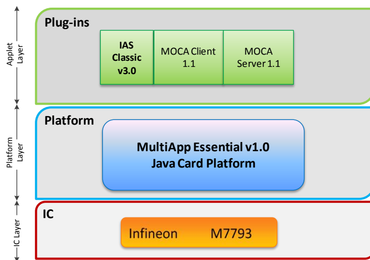
Figure 1: MultiApp Essential V1.0 smartcard architecture
