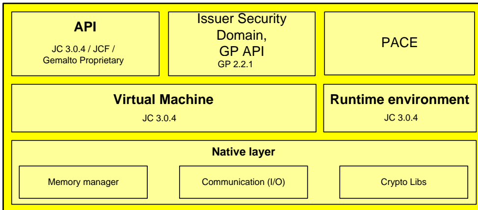
Figure 3: MultiApp Essential V1.0 Java Card platform architecture
