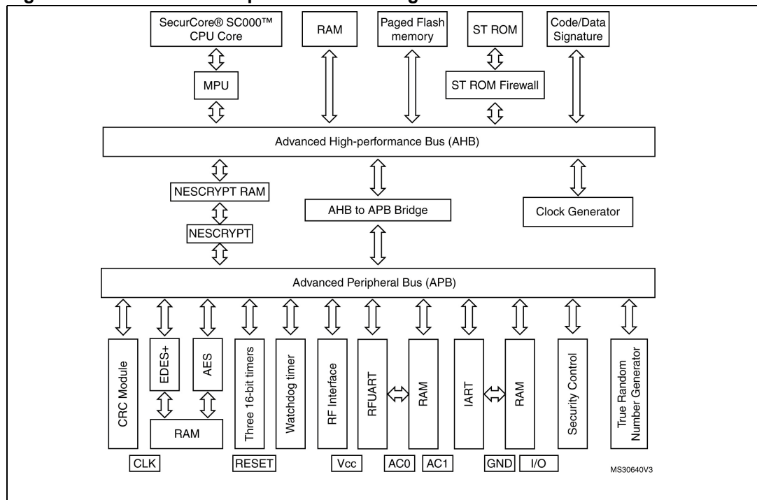
Figure 1. ST31G480 B02 platform block diagram
