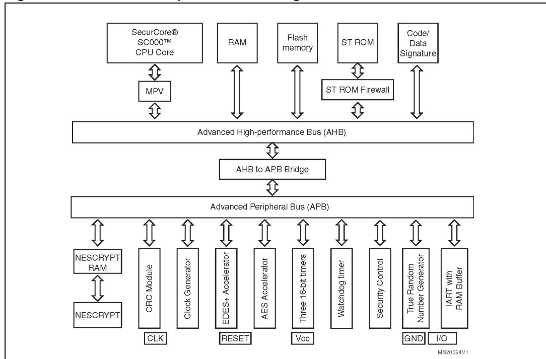
Figure 1. ST31H320 D01 platform block diagram
