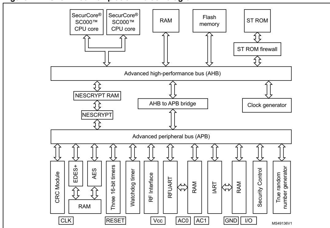
Figure 1. ST31P450 A04 platform block diagram
