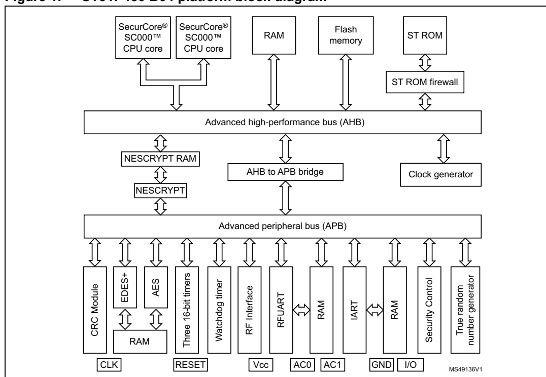
Figure 1. ST31P450 B04 platform block diagram
