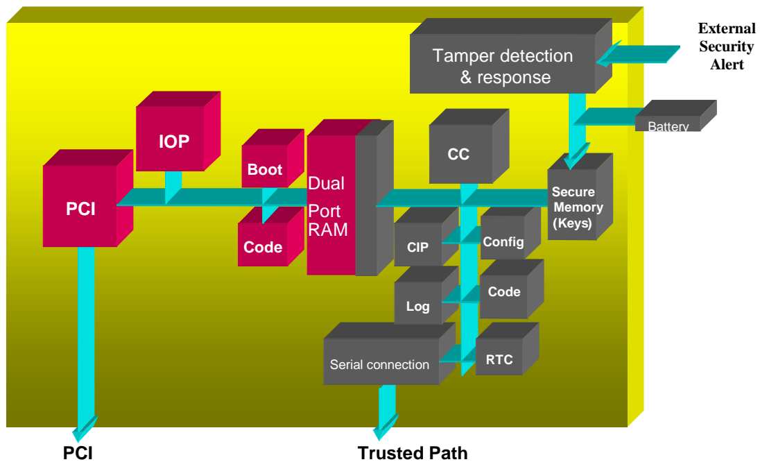
Figure 1: TOE Architecture
