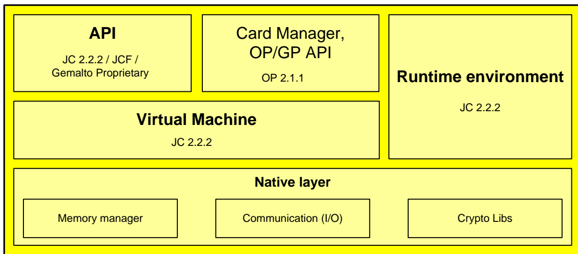
Figure 3: MultiApp ID V3.1 javacard platform architecture
