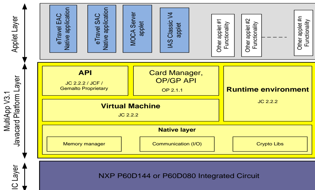
Figure 1: MultiApp ID V3.1 smartcard architecture
