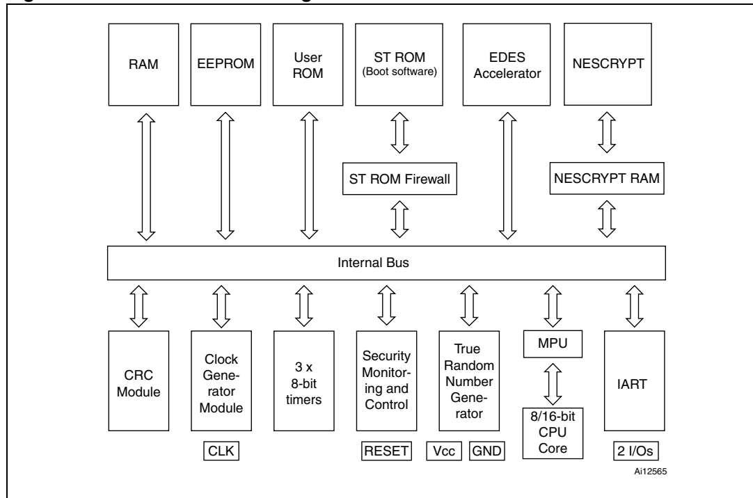
Figure 1. SA23YL80B block diagram
