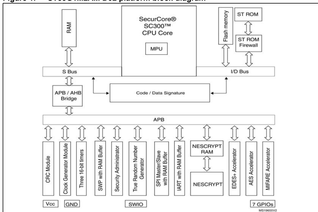
Figure 1. ST33G1M2AM D02 platform block diagram
